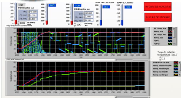
Management and control system for hydrogen processor
